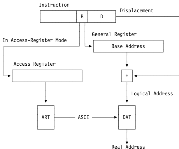
Figure 5-8. Use of Access Registers
